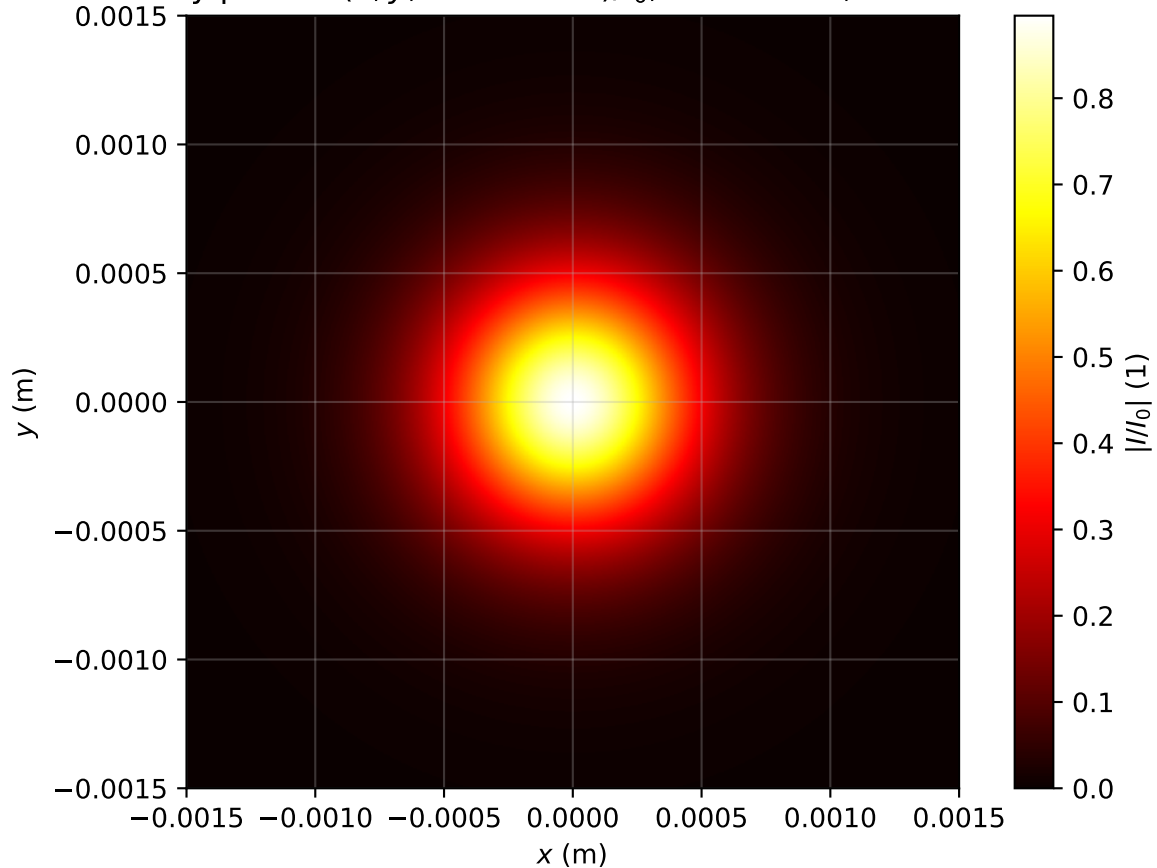
Intensity profile I(x, y, z = 2.786m)/I_0 , \text{Pin}=0.7\text{Pcr} , artificial time
